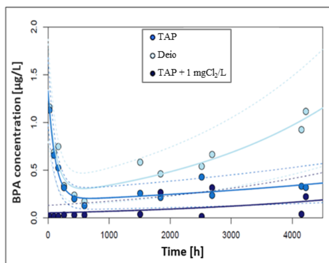
Fig. 6. BPA migration over time: dots correspond to experimental data as a function of the tested water matrix. Solid lines indicate the estimated models, dashed lines represent the models 95% confidence intervals [8].
