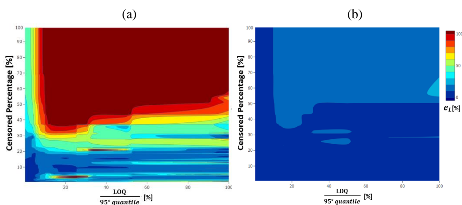
Fig. 2. Contour plot of the estimation error ( e_L ) of health risk as a function of the percentage of censored data and amplitude of data range for elimination (a) and MLE_{LC} (b) methods [2].
