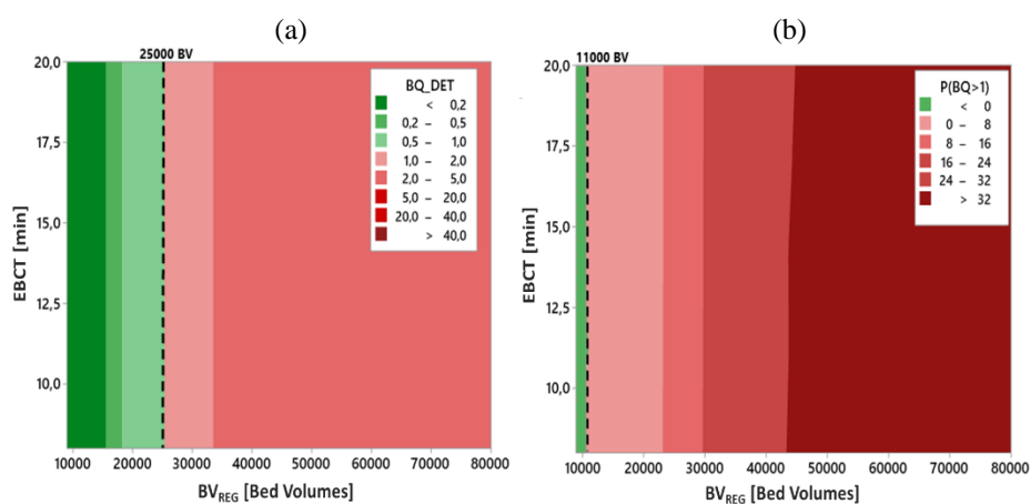
Fig. 3. Contour plot of BQ_{DET} (a) and P(BQ > 1) (b) as a function of the empty bed contact time (EBCT) and the regeneration time ( BV_{REG} ) [5].
