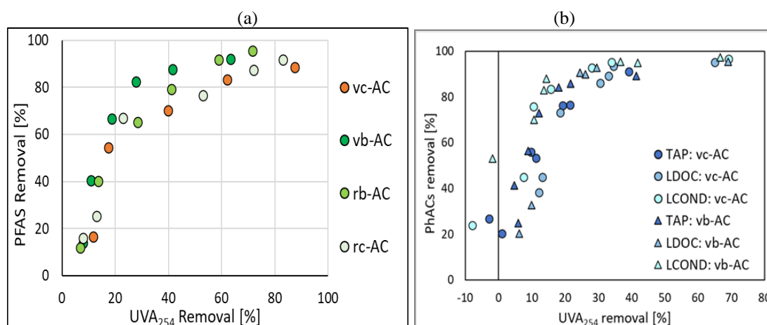
Fig. 5. Correlations between: (a) overall PFAS removal (a) and UVA_{254} removal as a function of the four tested ACs [6], (b) overall PhACs removal and UVA_{254} removal as a function of two tested ACs and three water matrices.
