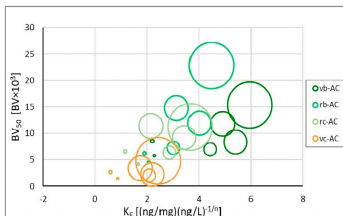
Fig. 4. Bubble chart for PFAS removal by adsorption on activated carbon (AC). Bubble centers are located according to the isotherm K_F and the RSSCT BV_{50} ; bubble diameters are proportional to respective PFAS hydrophobicity [6].
